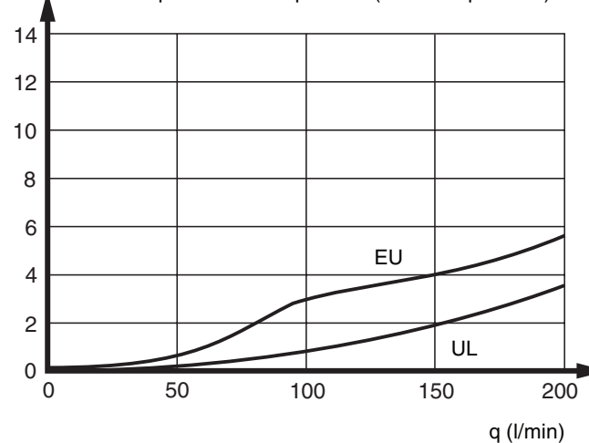
\Delta p (bar) Pressure drop pump-to-tank for unloaded valve. Spool in neutral position (no-load operation).
