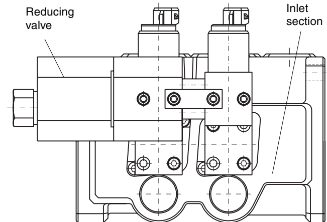
ESO/ESP on more than one spool section. No connection S [49]. Reducing valve R for item [50]. With R as item [50], reducing valve's pump and tank connection are turned in toward the directional valve.
