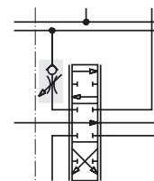
Adjustable restrictor and check valve in pressure gallery (MS or A16)
