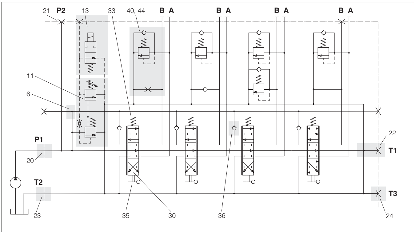
Diagram shows one H170CF with four spool sections.
