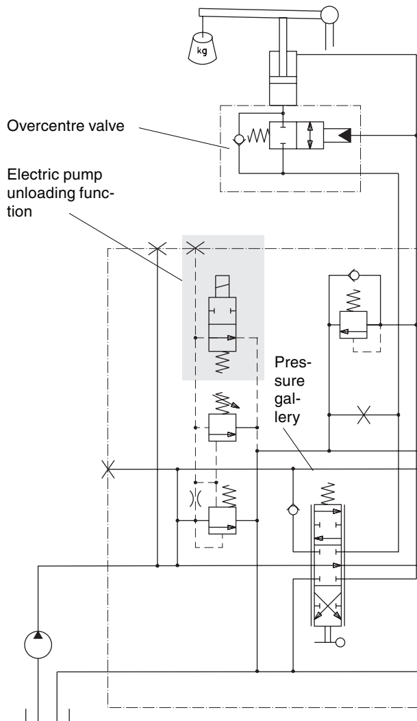
Connection example that gives emergency STOP function
