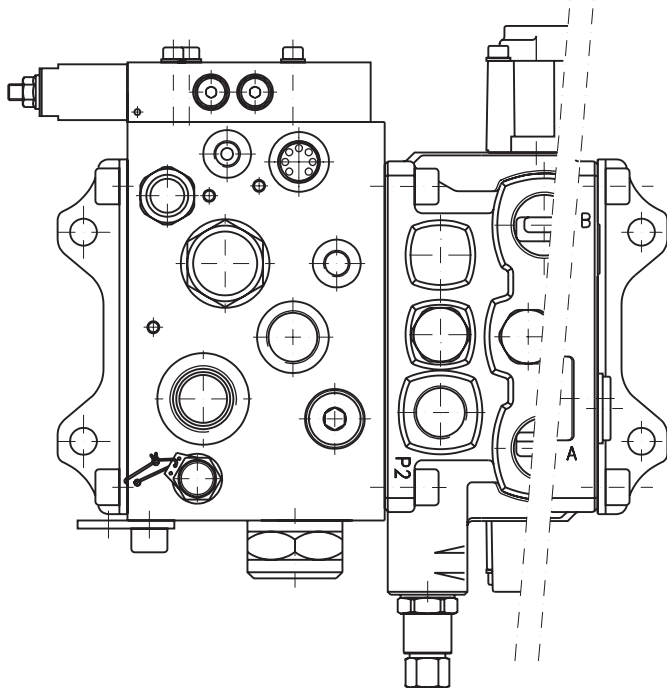
Above is an example of a specially customized function block. Like most function blocks, it was constructed using cartridge valves, i.e. only the housing is a unique component.
