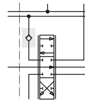
Check valve in pressure gallery (NS)
