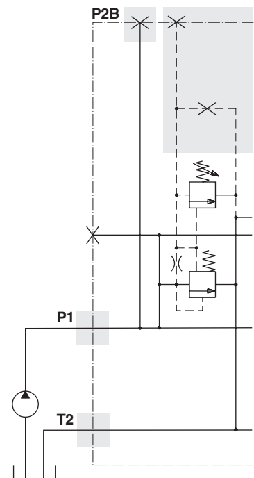
Inlet without unloading function (code ULB).
