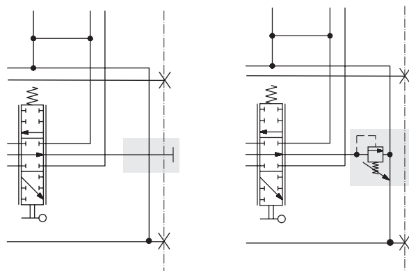
Tank connection T1 fitted with S-nipple. Free-flow gallery not connected with tank.
