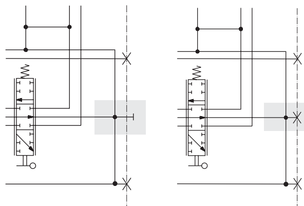
Tank connection T1 open (T1). Free-flow gallery connected with tank.
