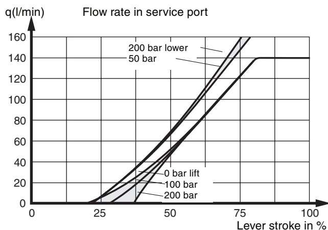
Remote controlled DPC spool, Q140. In H170CF valves with closed spool actuators (PC), the spools are pressure compensated, with the result that the load's effect on speed is minimal.
