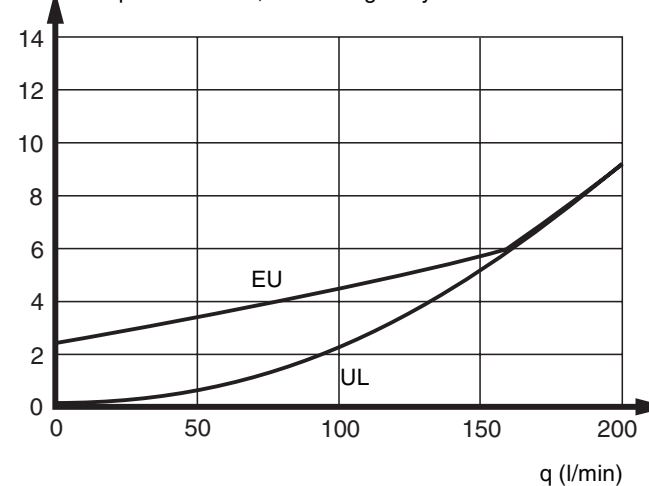
\Delta p (bar) Pressure drop pump-to-tank on emergency unloading. Spool actuated, free-flow gallery blocked.
