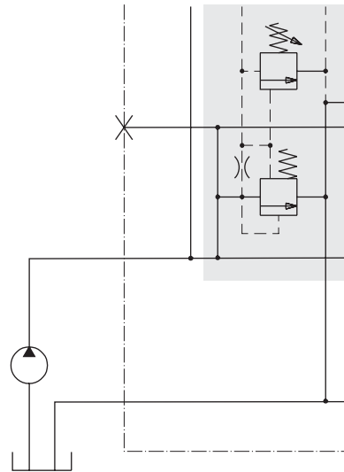
Inlet section with main pressure relief valve PS or PB.
