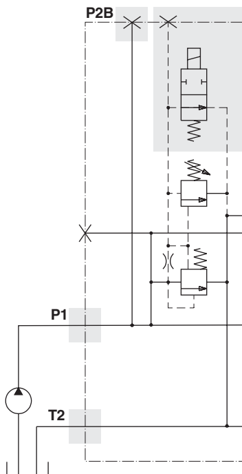
Inlet equipped with EU12/EU24 electric pump unloading. Energising the solenoid closes the unloading valve.
