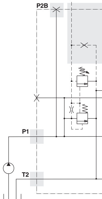
Inlet fitted with UL nipple and an external pilot circuit. The external pilot circuit contains a valve that opens a connection to a pressure relief valve on receipt of a signal. The setting on this pressure relief valve should be lower than the setting on the main pressure relief valve that is built into the directional valve. In this way, a two-level pressure relief function is obtained.
