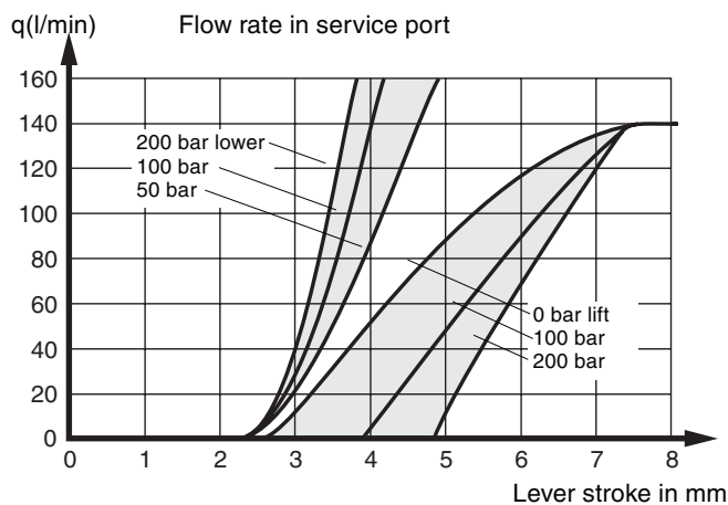
Hand operated D-spool, Q140. In H170CF valves with hand-operated spools, speed is affected by the weight of the load, i.e. the heavier the load, the longer the lever stroke needed before the load starts to move.
